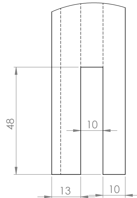
DETAIL B SCALE 1 : 1
